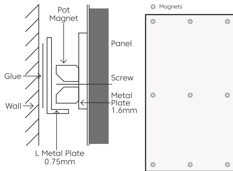
Pot Magnet Install
