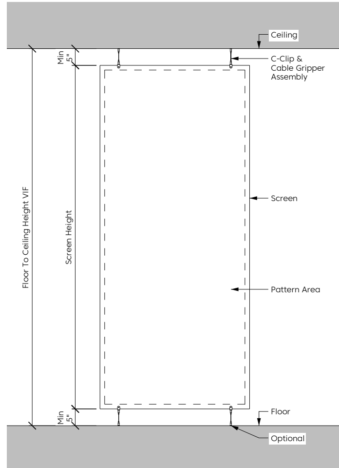
Cable Hanging System
