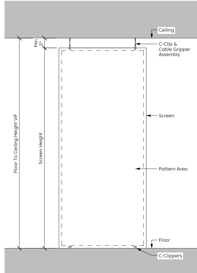
Cable Hanging System With C-Clippers
